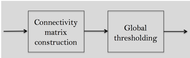
Fig. 1: Classical framework.
