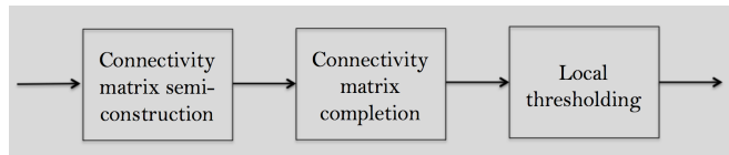
Fig. 2: Proposed framework.
